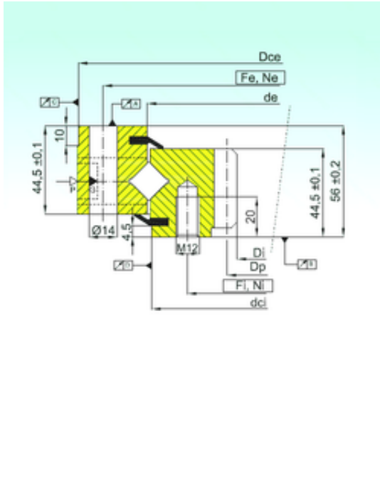
ZR1.14.0744.201-3SPTN Bearing 2D drawings and 3D CAD models
