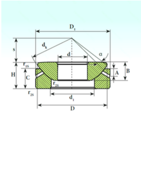
GX 40 S Bearing 2D drawings and 3D CAD models
