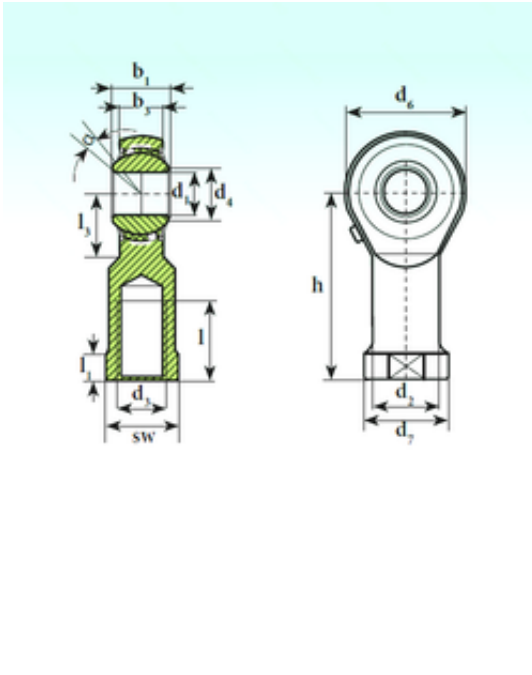
TSF 12 BB-O Bearing 2D drawings and 3D CAD models
