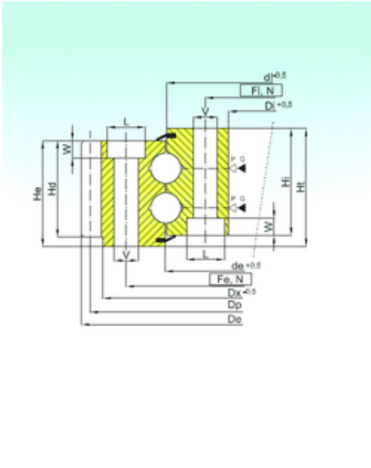
EB2.25.0475.200-1SPPN Bearing 2D drawings and 3D CAD models
